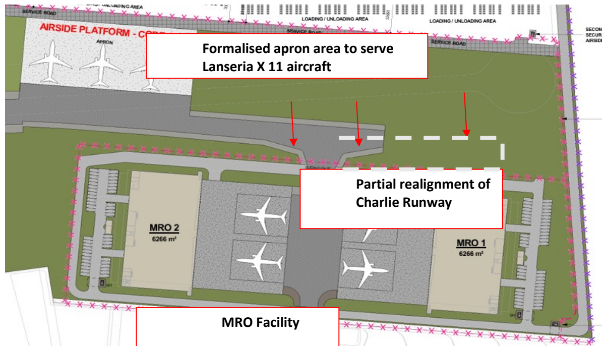
Figure 2: Project layout, indicating the partial-realignment of the Charlie
